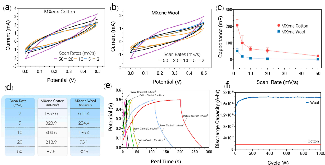
Fig. 5. CV curves of a) cotton and b) wool TSCs at various scan rates; c) specific capacitance of cotton and wool TSCs at various scan rates; d) a table of values calculated for the specific areal capacitance of cotton and wool TSCs; e) GCD curves of cotton and wool at various current densities; f) CDC cycles of cotton and wool TSCs to compare cycle life of the two substrates.
