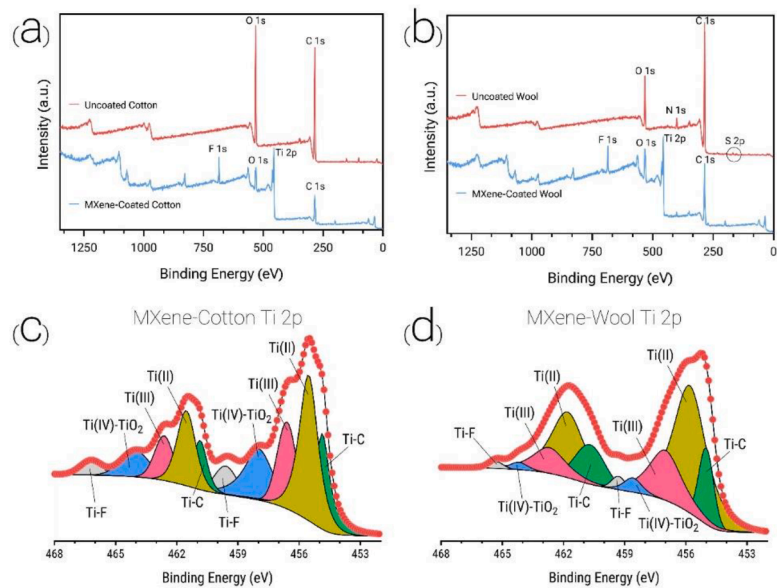
Fig. 2. XPS surveys of MXene-coated and uncoated a) cotton and b) wool yarn; high-resolution Ti2p spectra of MXene-coated c) cotton and d) wool yarn.
