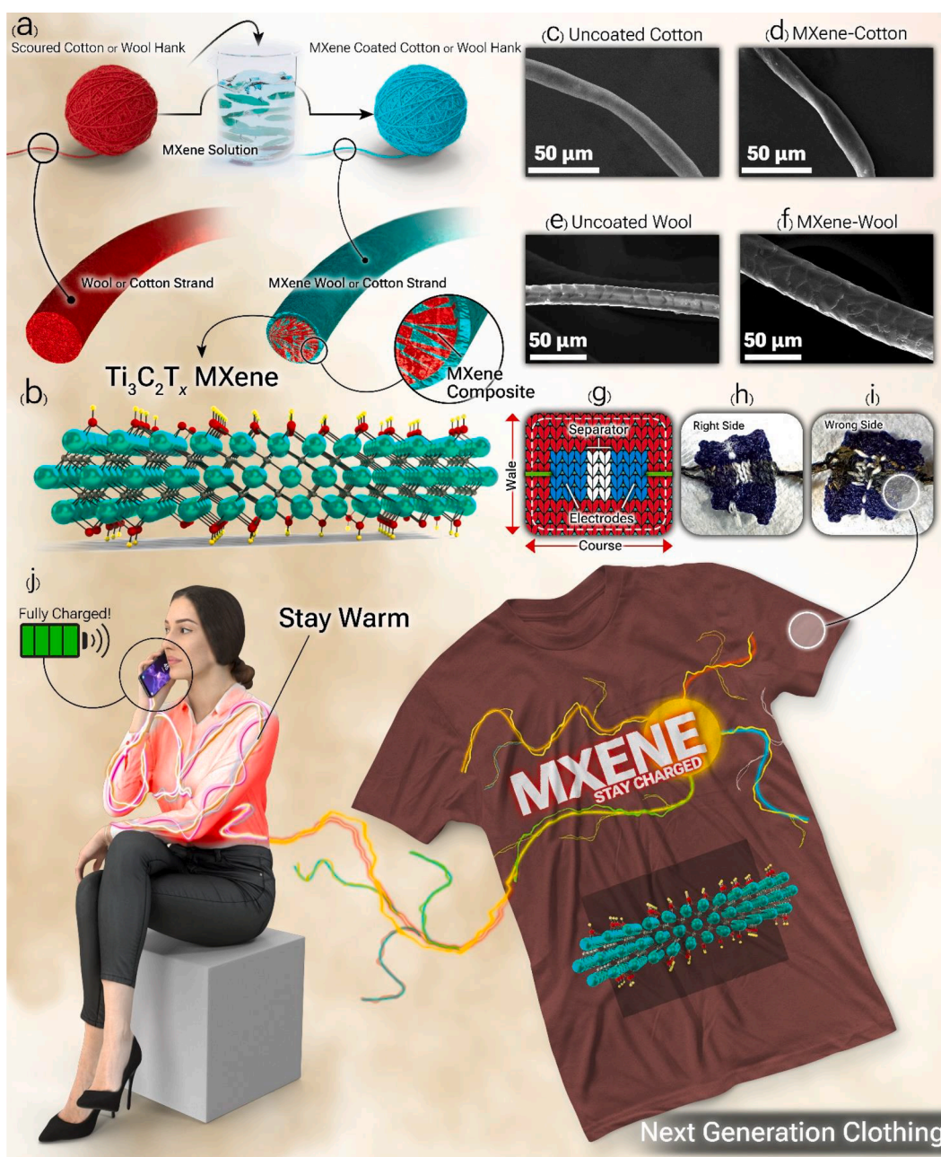
Fig. 1. a) Showing the coating of MXene flakes on cotton or wool yarn; b) \text{Ti}_3\text{C}_2\text{T}_x MXene flake atomic structure; SEM images of c) uncoated cotton; d) MXene-coated cotton; e) uncoated wool; f) MXene-coated wool; g) geometry of knitted TSC with course and wale directions defined; h) right side of knitted TSC; i) wrong side of knitted TSC; j) conceptual design of smart energy storing garment.
